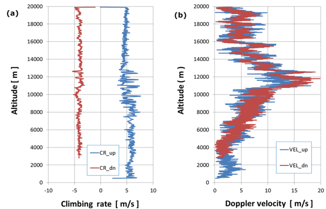
Figure 10. Double balloon flight to 20 km and back. Panel (a) shows the ascent and descent rates as functions of altitude. Panel (b) shows the Doppler velocity with considerably less noise during the descent than during the ascent, which demonstrates that for the double ballooning method, the descent is more quiescent than the ascent.
