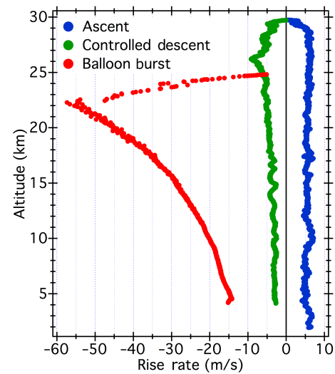
Figure 1. Typical balloon vertical velocities during ascent (blue) followed by controlled descent using the automatic valve method (green) or descent after balloon burst (red). The ascent profile shows the valve opened at 28.5 km, first reducing the ascent rate to zero (float) then establishing a slow and fairly steady descent rate < 10 \text{ m s}^{-1} (green). The red profile indicates the balloon burst prematurely at 25 km, prior to activation of the valve. The descent rate after burst initially exceeded 50 \text{ m s}^{-1} then was gradually slowed to < 20 \text{ m s}^{-1} by the parachute. For both descent profiles reception of the radiosonde telemetry signal was lost at \sim 4 \text{ km} .
