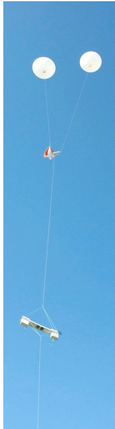
Figure 8. Flight configuration for the double balloon method. Each of the two balloons and payload are attached to a vertex of a triangular aluminium frame outfitted with the Intelligent Balloon Release Unit that releases the carrier balloon at a preset altitude. The configuration is shown attached to the launching pole just prior to release.
