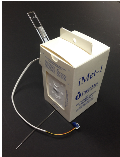
Figure 11. Internet iMet-1-RS radiosonde used for FPH flights at Boulder.
