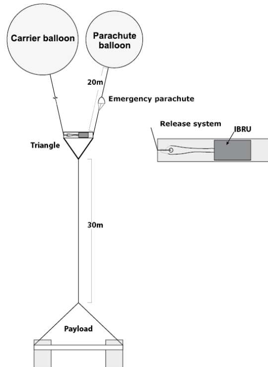
Figure 6. Double balloon sounding configuration with carrier and parachute balloon connected to the payload via the triangle that includes the IBRU release mechanism.
