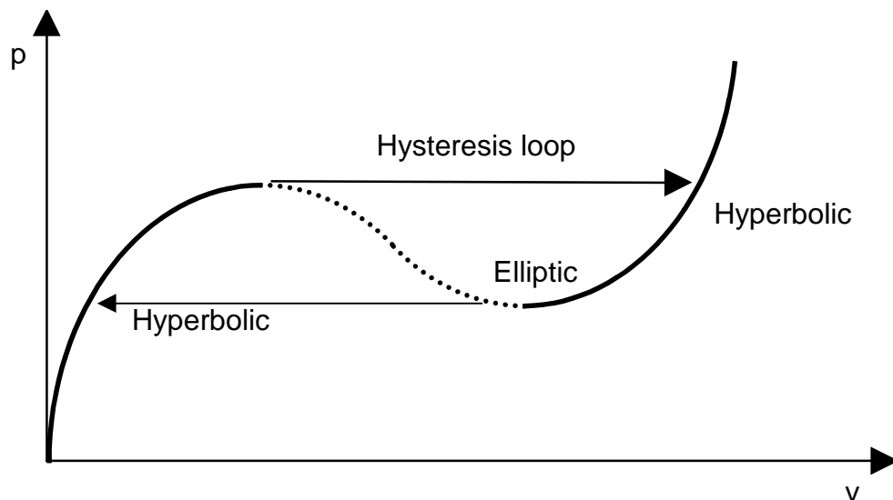
Figure 9.1. The system (9.1) is hyperbolic when p'(v) > 0 . The elliptic branch is unstable in the sense of Hadamard. This region is called “spinoidal”.
