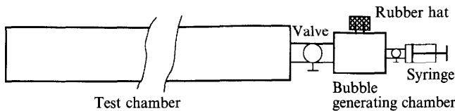
FIGURE 3. Two-chamber system. The test air bubble is generated in a separate small chamber which is connected to the test column through a valve.
