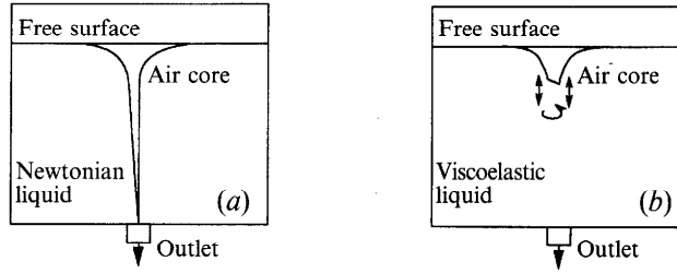
FIGURE 12. Sink flow of (a) a Newtonian liquid and (b) a viscoelastic liquid. In the viscoelastic case, an inclined two-dimensional cusp with a guillotine edge develops at the place where the air core disappears. This cusp rotates around its axis as it fluctuates up and down. We could imagine this cusp on an air bubble held in place by withdrawing liquid.
