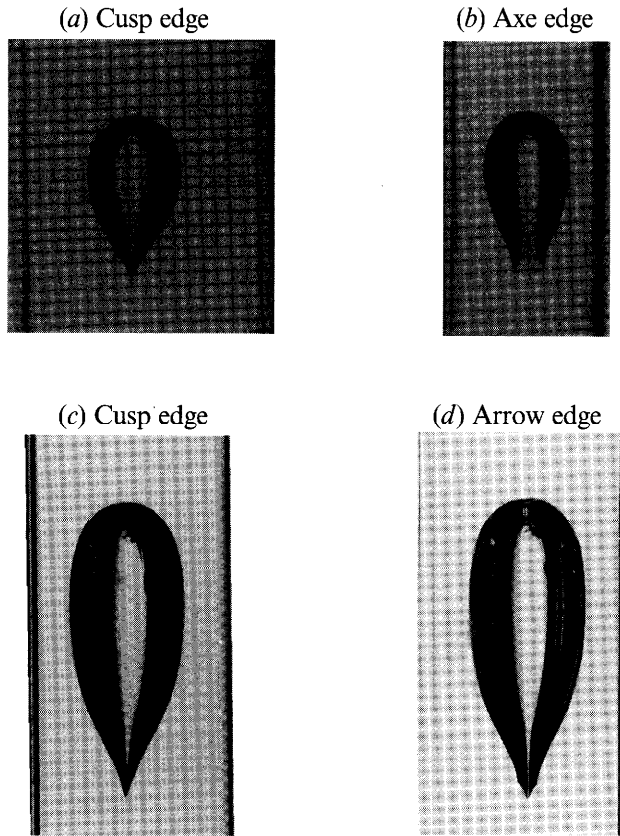
FIGURE 10. Cusped air bubbles rising in S1. (a) A 2\text{ cm}^3 bubble photographed from the wide side of the rectangular bubble column 1. (b) Photographed from the narrow side of column 1. (c), (d) Photographs of a 6\text{ cm}^3 bubble in the square bubble column 2 from mutually perpendicular directions.
