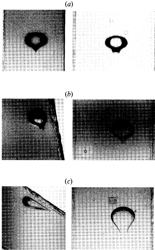
FIGURE 15. Two-dimensional cusps in inclined columns: 10 \text{ cm}^3 bubbles rising in 1.5% polyox in the rectangular column 7. Photographs on the left-hand side were taken from the narrow side of the column, and those on the right from the wide side. (a) Vertical column (supercritical), (b) column tilted 80^\circ from horizontal (subcritical), (c) column tilted 40^\circ from horizontal (wall dominated). The change in orientation which was caused by tilting through 80^\circ is remarkable.
