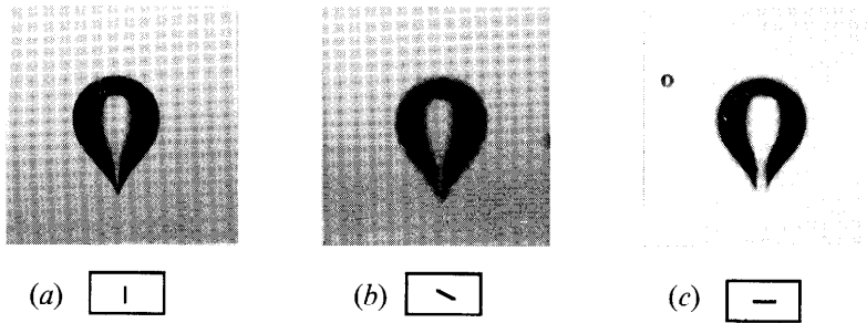
FIGURE 14. Metastable orientations in regime 2 of a 0.5 \text{ cm}^3 air bubble rising in 1% solution of polyox in water in rectangular column 4: (a) parallel to the narrow window, (b) on the diagonal and (c) perpendicular to the narrow window. The orientation is also indeterminate when the sidewalls are far removed.
