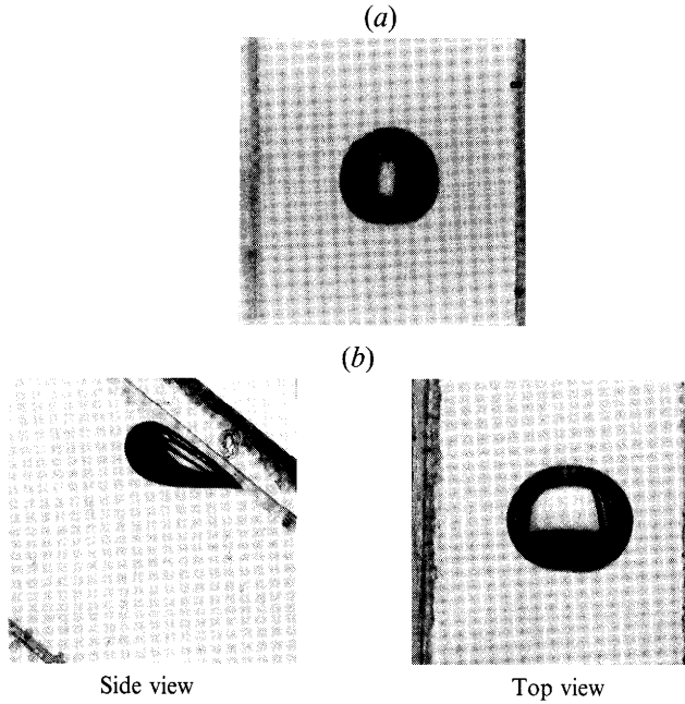
FIGURE 17. An air bubble rising in glycerin in a vertical column does not cusp (see a for a 0.45 cm 3 bubble), but it does cusp when it is sheared against a tilted wall with tilt angle between 20° and 75°, as shown in ( b ) for a 1 cm 3 bubble rising in a 45° tilted column.
