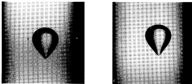
FIGURE 11. An air bubble of volume 0.5\text{ cm}^3 rising in a 1.5% solution of polyox in water. The photographs were taken from two mutually perpendicular directions in round column 6.
