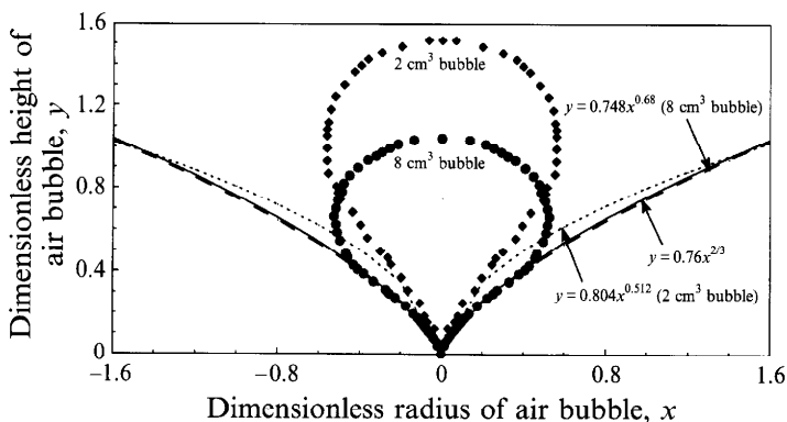
FIGURE 16. Analytic approximations of the cusp shape for the 2 \text{ cm}^3 and 8 \text{ cm}^3 bubbles shown in figure 7. The radius and height of the bubbles are made dimensionless with their equivalent diameters. The cusp is fitted to a power law whose index increases asymptotically to 2/3 as the bubble volume increases.
