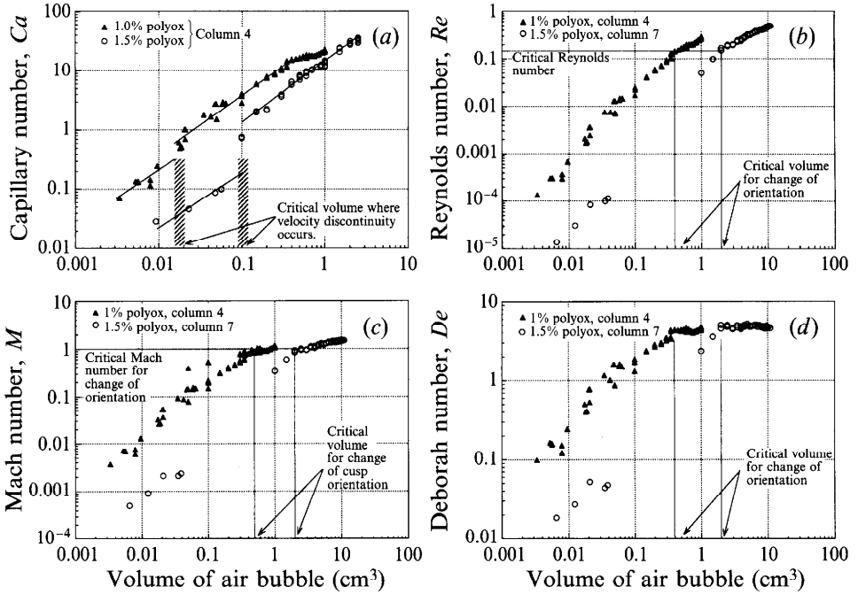
FIGURE 4. Rise curves: volume of air bubble vs. (a) Ca , (b) Re , (c) M and (d) De . A terminal velocity U > c could not be achieved in the 1.5% polyox solution when the column 4 diameter was too small but we did obtain bubbles of large volume with U > c , but not too large to measure in the larger column 7. Critical volumes for discontinuities of value and slope of the rise curves are indicated.
