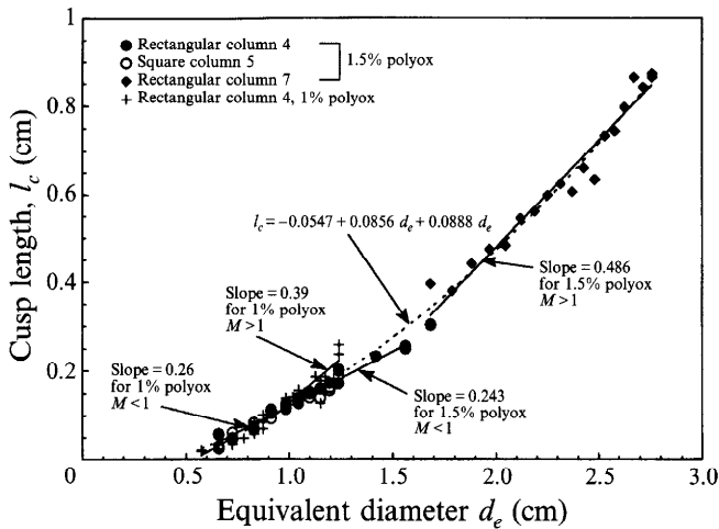
FIGURE 9. The relation between cusp length and equivalent diameter of an air bubble in 1% and 1.5% aqueous polyox solutions in various columns.
