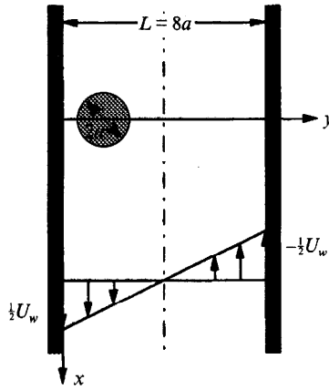
FIGURE 1. Migration of a particle in a simple shear flow between walls. \kappa = 0.125 , \mathcal{R}_p = 0.625 .
