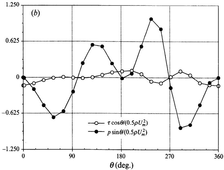
FIGURE 20. Distributions of pressure and viscous stresses on the surface of a neutrally buoyant particle in a Poiseuille flow. R_p = 3.125 . The position of the particle is (x, y) = (19.82, 0.3628) L , which is marked by a circle in figure 17. (a) Pressure and shear stress; (b) horizontal projections. Because of the definition of \theta , positive projection corresponds to lateral thrust toward the left wall. The resultant lateral forces (scaled by the inertial force \rho U_m^2 a ) are: F_p = -3.67 \times 10^{-3} , F_r = -6.725 \times 10^{-4} .
