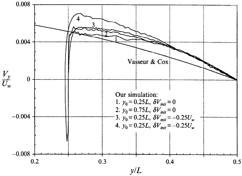
FIGURE 4. Comparison of the migration velocity predicted by our simulation and the theoretical result of Vasseur & Cox (1976) for small spheres. The centreline of the channel is at y = 0.5L . The sign of V_y for curve 2 has been changed for comparison. The particle Reynolds number is 1.25 for curve 4 and is 0.625 for the other three curves.
