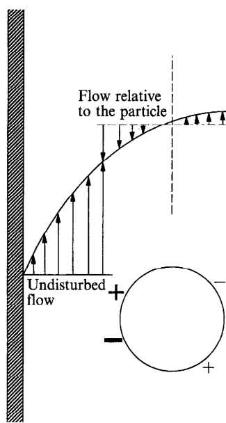
FIGURE 19. Cartoon showing the relative flow and pressure extrema around a neutrally buoyant particle in a Poiseuille flow. The particle is in a position marked in figure 17. R_p = 3.125 .
