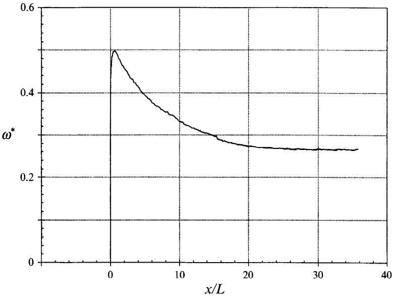
FIGURE 10. The angular velocity (made dimensionless by the shear-rate \omega^* = \omega L/U_w ) of a slightly buoyant particle decreases as it approaches the wall. \rho = 0.998 , final lead R_{slip} = 0.057 .
