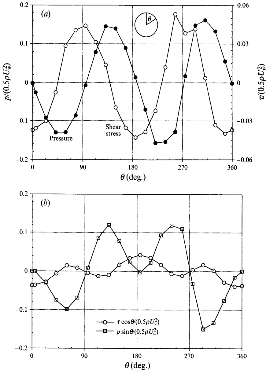
FIGURE 6. Distribution of pressure and viscous stresses on the surface of the particle at an early time of migration (curve 1 in figure 2). t^* = 1.479 , (x, y) = (0.2895L, 0.25275L) . (a) Pressure and shear stress; (b) horizontal projections. Because of the definition of the angle \theta , negative projection corresponds to lateral lift in the positive y -direction (to the right). The resultant lateral thrusts per unit length (scaled by the inertial force \rho U_w^2 a ) are: F_p = 7.842 \times 10^{-3} , F_\tau = 5.238 \times 10^{-3} .
