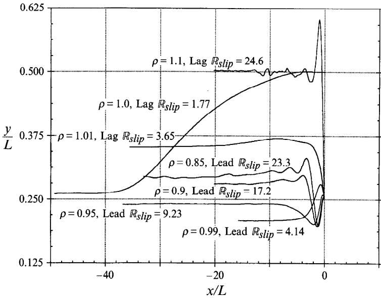
FIGURE 21. The migration of buoyant particles in a plane Poiseuille flow. \mathcal{R}_b = 120 , \mathcal{R}_p = 1.875 , F_r = 43.56 . Initial position y_0 = \frac{1}{4}L except for the neutrally buoyant case shown here for comparison.
