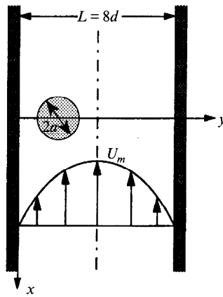
FIGURE 15. Geometry for the migration of a particle in a plane Poiseuille flow.
