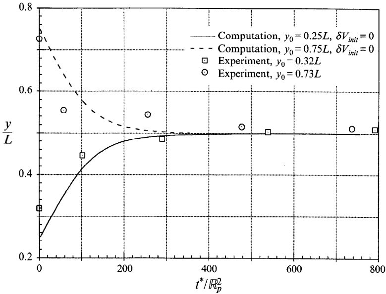
FIGURE 5. Particle trajectories predicted in our simulation compared to those observed by Halow & Wills (1970 b ) in a cylindrical Couette device. In the computation, R_p = 0.625 , \kappa = 0.125 . In the experiment, R_p = 1.601 , \kappa = 0.179 .
