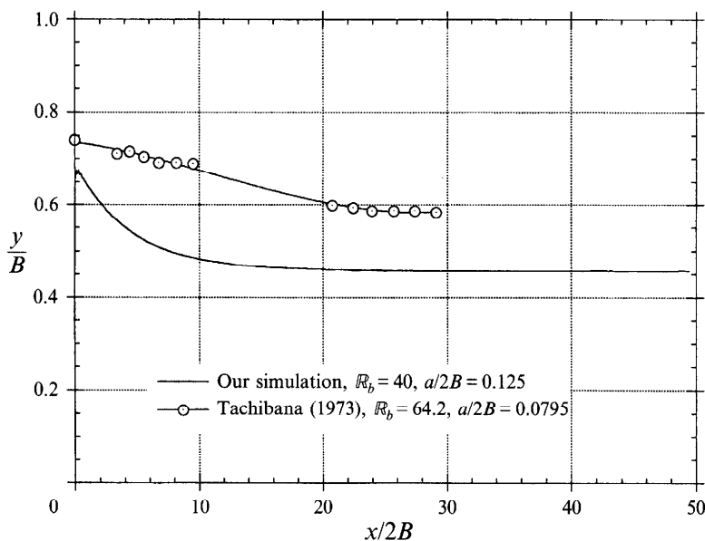
FIGURE 23. Comparison of the simulated migration trajectory of a neutrally buoyant particle with the experiment of Tachibana (1973). The width of the column is 2B , and the centreline is at y = 0 . The bulk Reynolds number is defined as R_b = 2U_m B/\nu .
