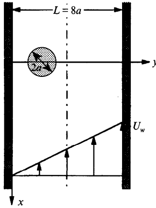
FIGURE 8. Migration of a buoyant particle in an upward Couette flow between walls.
