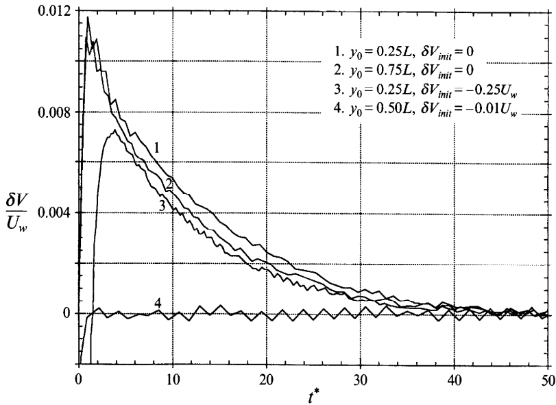
FIGURE 3. Relaxation of the slip velocity \delta V of particles migrating in a plane Couette flow. \delta V > 0 when the particle is leading the fluid in the left half ( y < \frac{1}{2}L ). The sign of \delta V has been changed for curve 2. The small wiggles are a numerical effect.
