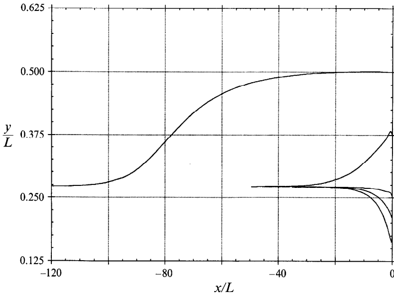
FIGURE 16. The Segré–Silberberg effect in a plane Poiseuille flow field. Particle Reynolds number R_p = 0.625 ; bulk Reynolds number R_b = 40 .
