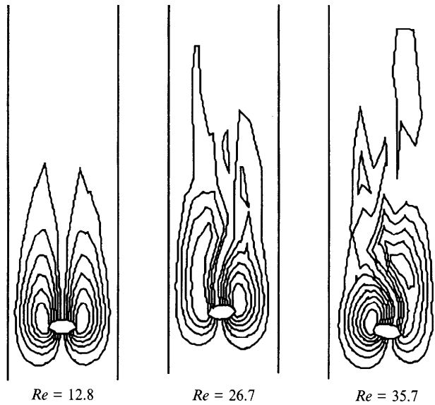
FIGURE 25. Streamlines around a 2:1 elliptic particle at different Reynolds numbers.
