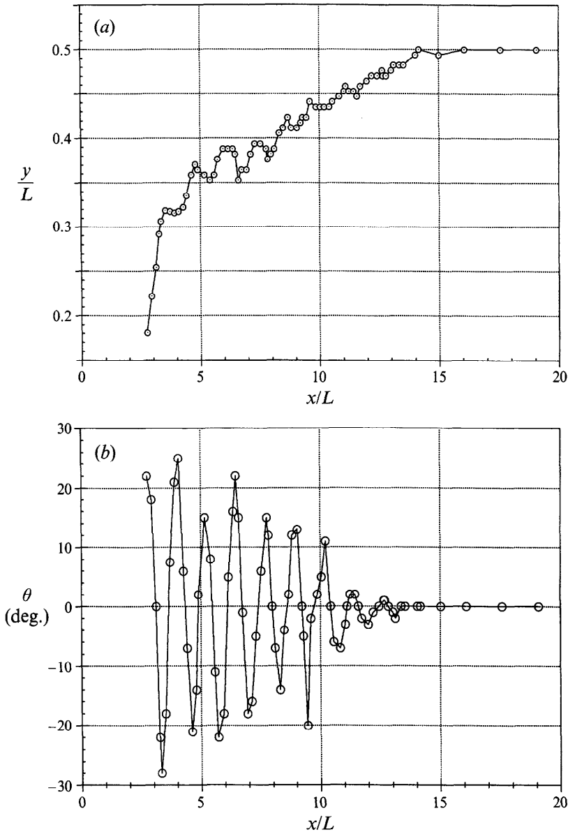
FIGURE 27. Sedimentation of a 2:1 elliptic cylinder in the wide 'two-dimensional' channel at Re = 694.7 . (a) Lateral position of the centre of the ellipse; (b) orientation of the cylinder ( \theta = 0 is with long axis horizontal).
