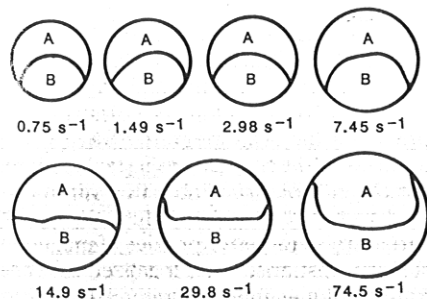
Fig. 1 Fluids A and B are viscoelastic fluids, and their viscosities vary depending on the apparent wall shear rate (given here in reciprocal seconds). In the upper set of arrangements, fluid B is the more viscous, and fluid A tends to wrap around fluid B. In the lower left, the viscosities of the fluids are about equal and the flat interface is retained. In the lower middle, fluid A is the more viscous and fluid B tends to wrap around fluid A. In the lower right arrangement, fluid A is the more viscous. (From J. H. Southern & R. L. Ballman Appl. Polymer Symp. 20 , 175–189; 1973.)
