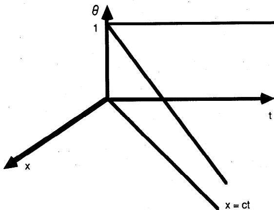
FIG. 1 Solution surface for Eq. (3.3) when \kappa_1=0 .
