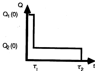
FIG. 4. Double step of relaxation.
