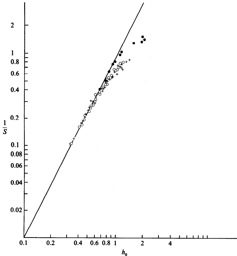
FIGURE 3. Comparison of the critical criterion (3.9) for run-off in coating flow with experiments. The solid line Sh_0^2 = 1 is theoretical: ●, silicone 1000 P; ○, STP 166 P; +, silicone 125 P.
