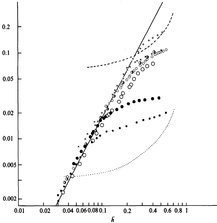
FIGURE 7. Comparison of the critical criterion (3.9) for run-off in rimming flow with experiments. The broken lines represent the line J = 4 for Soybean oil ( \cdots ) and Silicone 1000 ( --- ). The solid line Sh_0^2 = 1 is theoretical: +, STP; \bullet , Amoco oil, SAE 30; \times , Silicone oil, 12500 cp; \circ , Amoco gear lubricant 140; \circ , Silicone oil, 1000 cp; \bullet , Soybean oil; \bullet , Silicone oil 20 cp.
