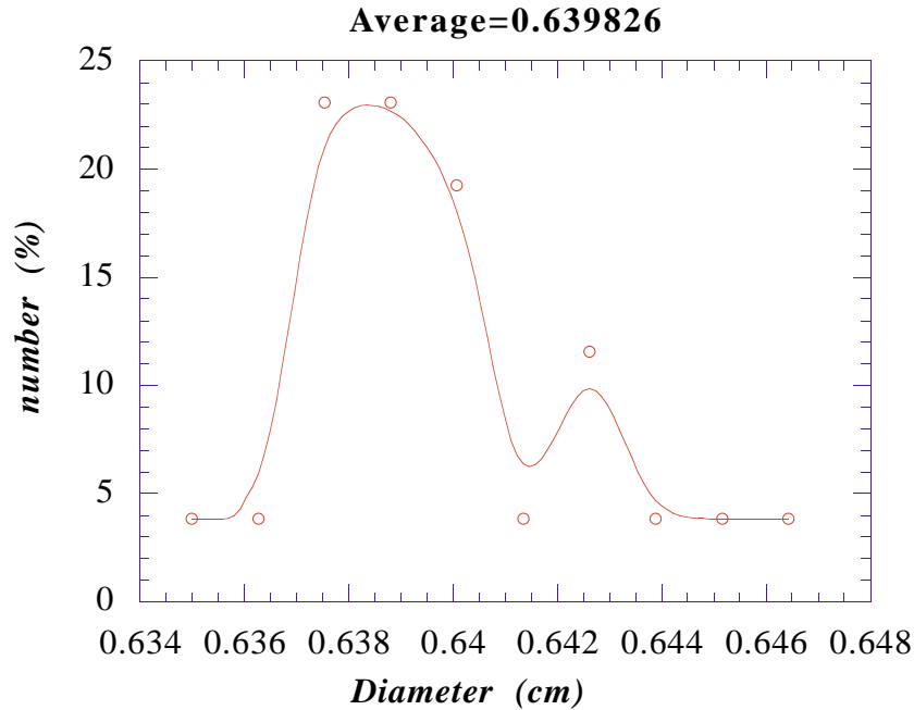
Figure 3. Distribution of diameter of spheres used in the fluidization experiment.
