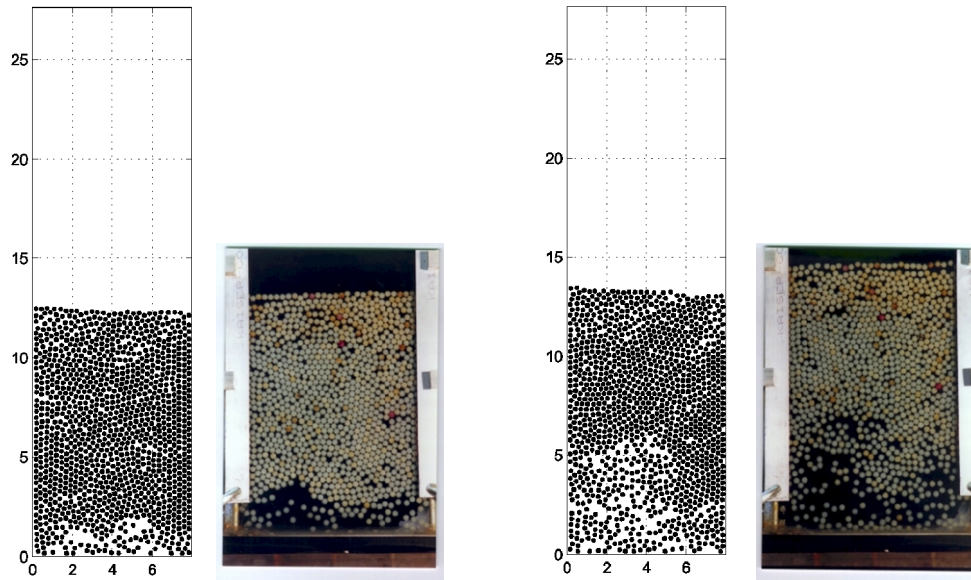
Figure 11. Comparison of snapshots of simulations of V = 4 at t = 2 (left) and 4 (right), and snapshots from experiments under equivalent conditions for the case of V = 4.037 .
