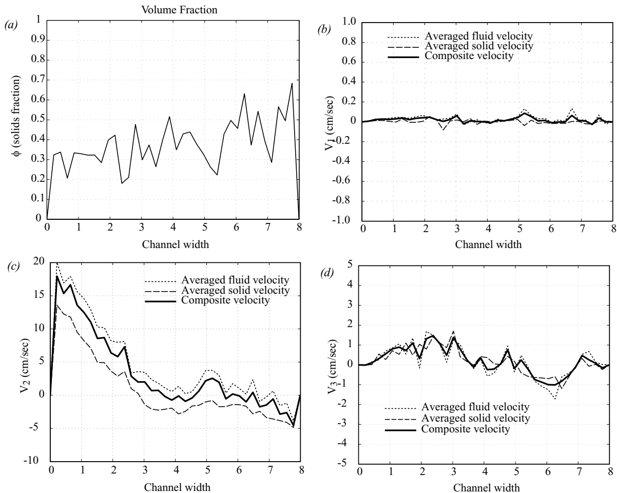
Figure 13. Volume fraction \phi and averaged components of velocity V_1, V_2, V_3 in coordinate direction x_1, x_2, x_3 at 38 nodes spaced at 1/10 in. across the 8 in. side of the fluidization column when V = 4.5 cm/s. (a) \phi , (b) V_1 , (c) V_2 , (d) V_3 . The difference between the averaged fluid and averaged solid velocity is the slip velocity. This is the first exact calculation of the slip velocity in a fluidized suspension.
