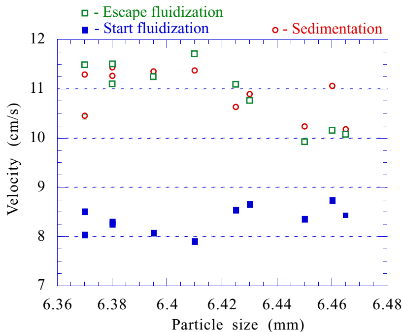
Figure 15. Sedimentation \circ and fluidization velocities \square \blacksquare from experiments using different size spheres. The particle lifts off the distributor when V is greater than \blacksquare and is dragged out of the column only when V is greater than \square .
