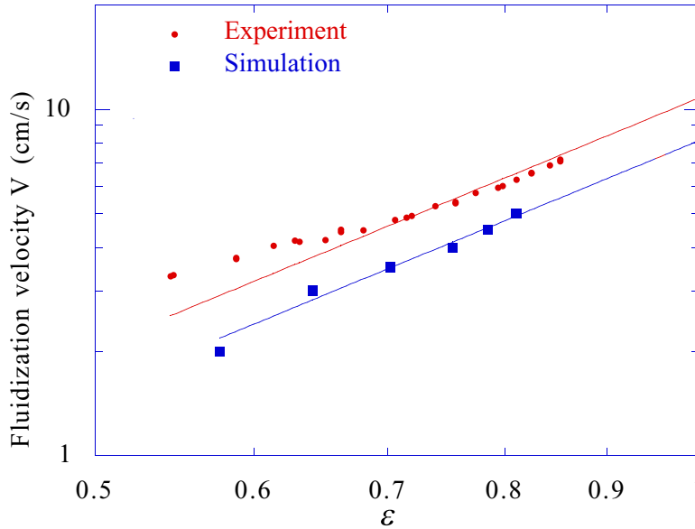
Figure 18. Data from Figure 17 plotted in a log-log plot. The slopes of the straight line are given by the Richardson-Zaki n = 2.39 . The blow-out velocities V_s(0) and V_e(0) are defined as the intercepts at \varepsilon = 1 .
