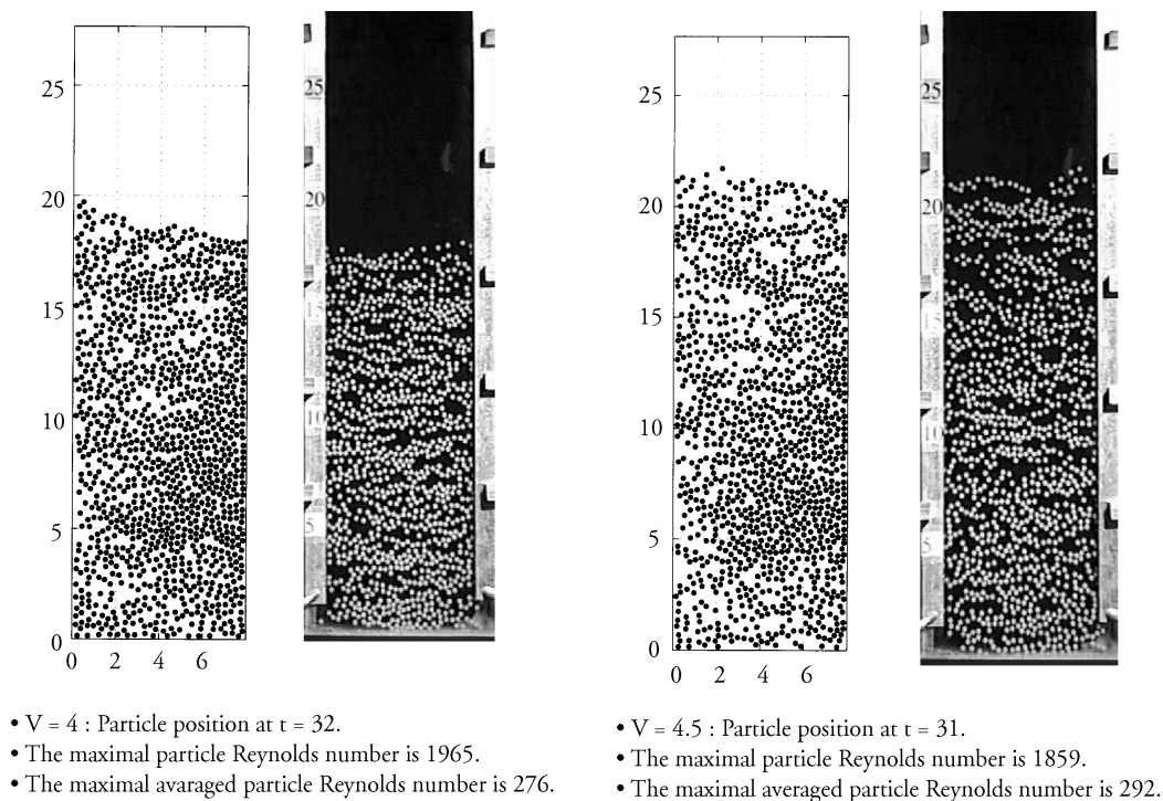
Figure 10. Cf. (c) in Figure 4 (left); cf. (d) in Figure 4 (right).
