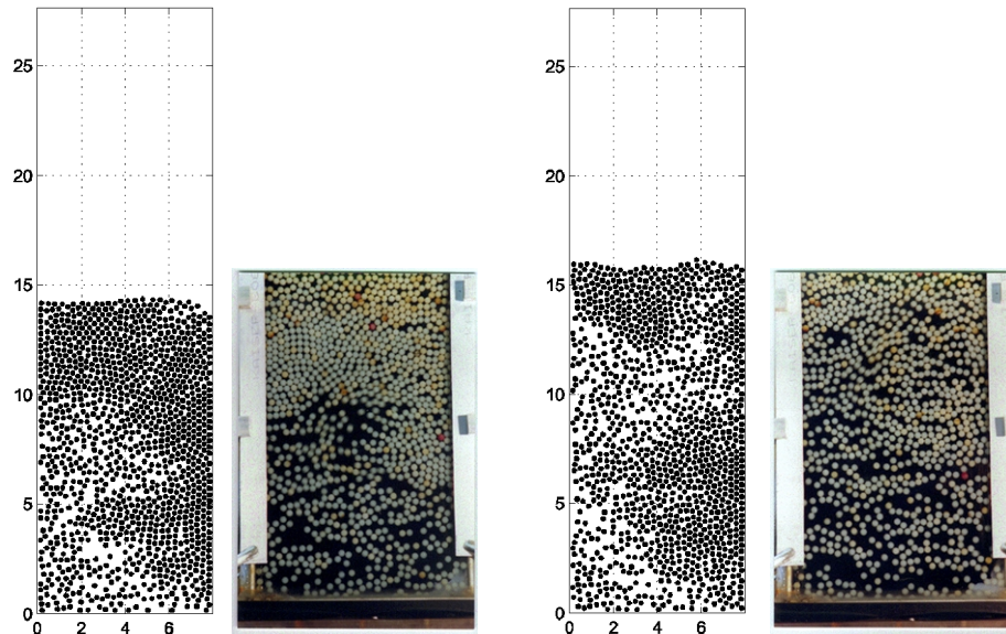
Figure 12. Comparison of snapshots of simulations of V = 4 at t = 6 (left) and 9 (right), and snapshots from experiments under equivalent conditions for the case of V = 4.037 .
