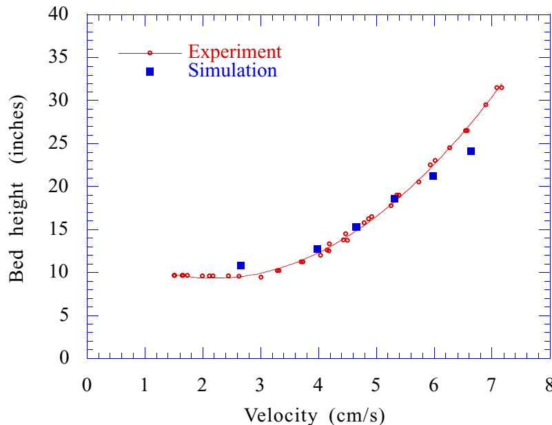
Figure 19. Bed height vs. fluidizing velocity after shifting by the ratio (9.8) of blow-out velocities obtained from the intercepts at \varepsilon = 1 in Figure 18.
