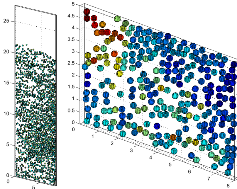
Figure 8. Snapshot of simulation of 1204 spheres with V = 4.5 (left) and a blow-up (right) at t = 31 .
