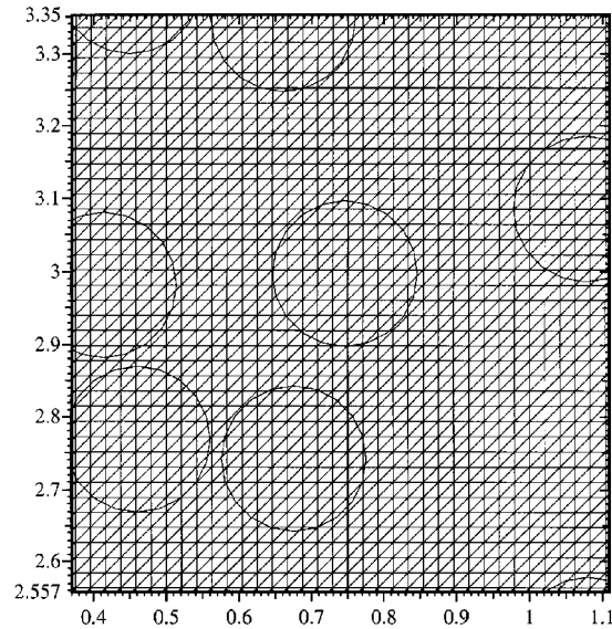
Figure 1. Part of a 2D example of a fixed triangular grid used in DLM computation. The same grid covers the fluid and solid. The fluid in the circle is bordered by Lagrange multipliers to move as a rigid body.
