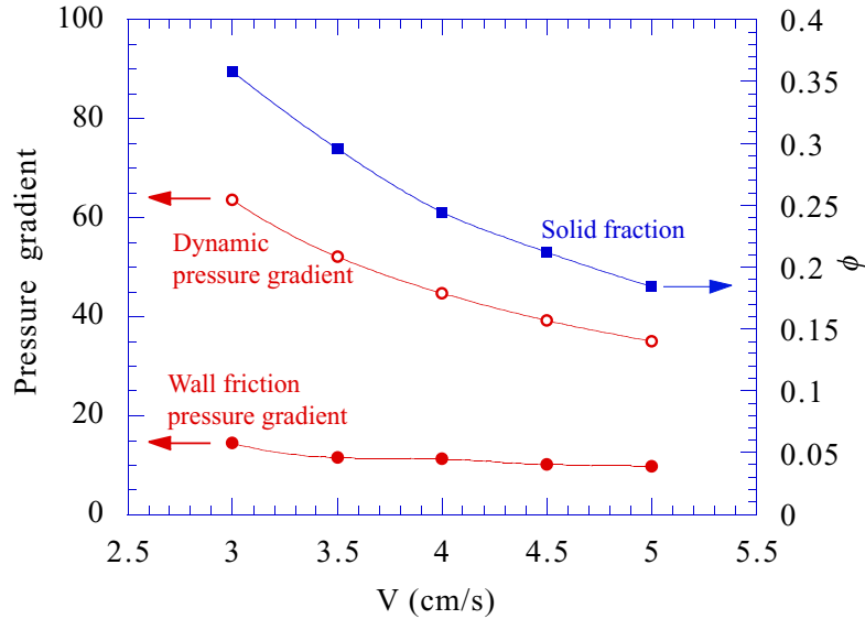
Figure 14. Solid fraction f dynamic pressure gradient and wall friction pressure gradient vs. fluidizing velocity.
