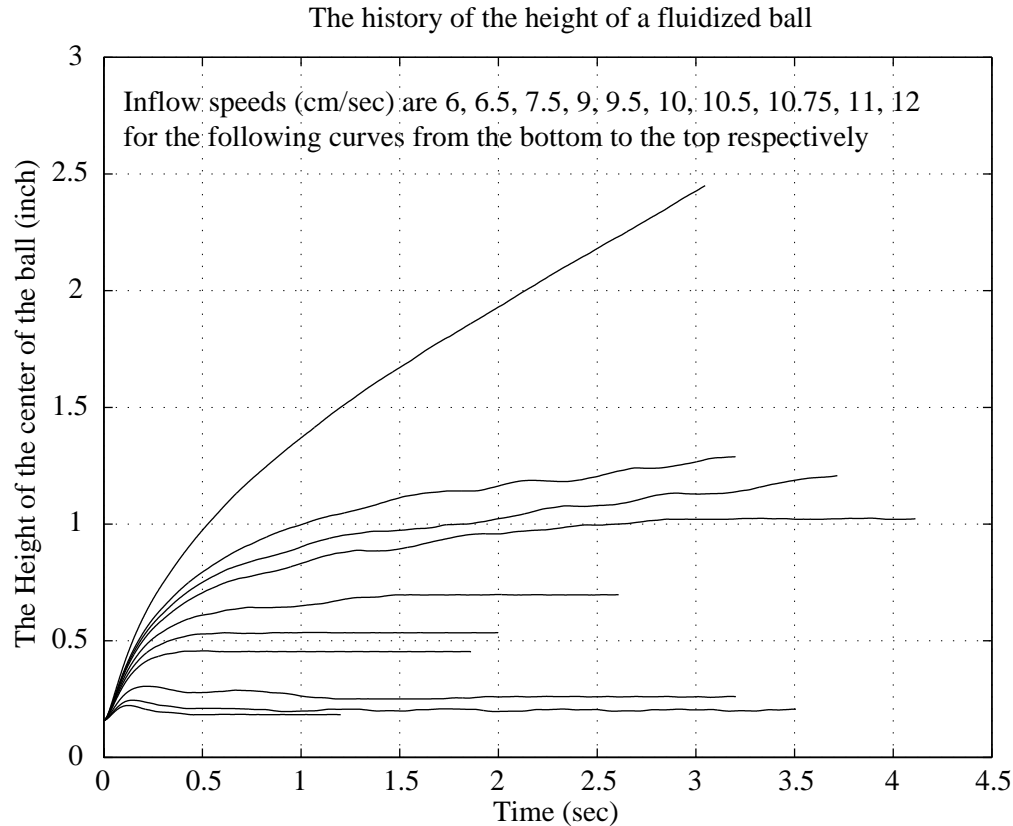
Figure 16. H vs. t for a single particle d = 0.635\text{cm} from numerical simulation. For V < V_m \approx 6\text{ cm/s} the sphere remains at the distributor; for V > V_m \approx 10.5\text{ cm/s} the sphere is dragged out of the bed.
