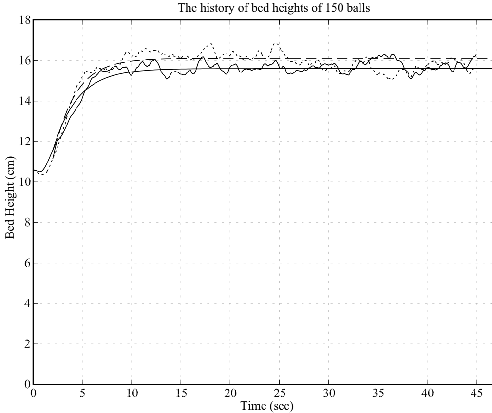
Figure 5. Bed height H vs. time for V = 4 cm/s. H(t) is the average height of the top layer of 150 spheres. The lines are least square fits to H(t) = a + b \exp(-c(t-2)) . Dashed - - - security zone 0.5h_v ; solid — security zone h_v .
