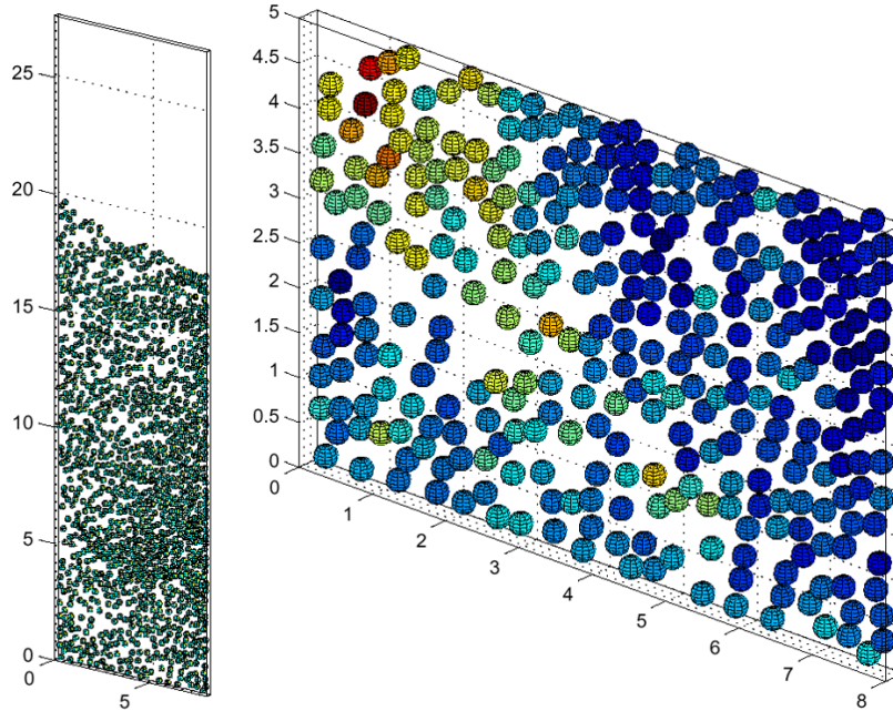
Figure 7. Snapshot of simulation of 1204 spheres with V = 4 (left) and a blow-up (right) at t = 32 .
