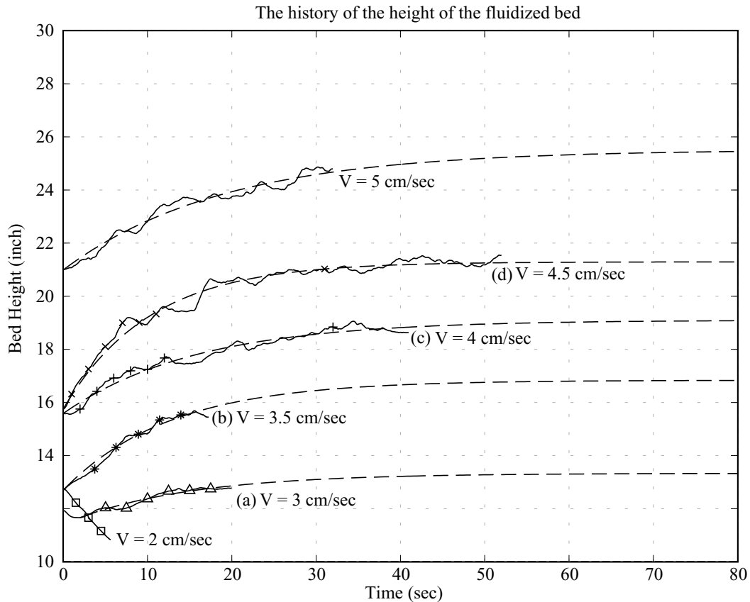
Figure 4. Bed height H vs. time for different values of the fluidizing velocity V . H is the average height of the top layer of 1204 spheres. The letters (a) ... (d) index the snapshots shown in Figures 9-10. The dashed lines - - - are least square fits to H(t) = a + b \exp(-ct) .
