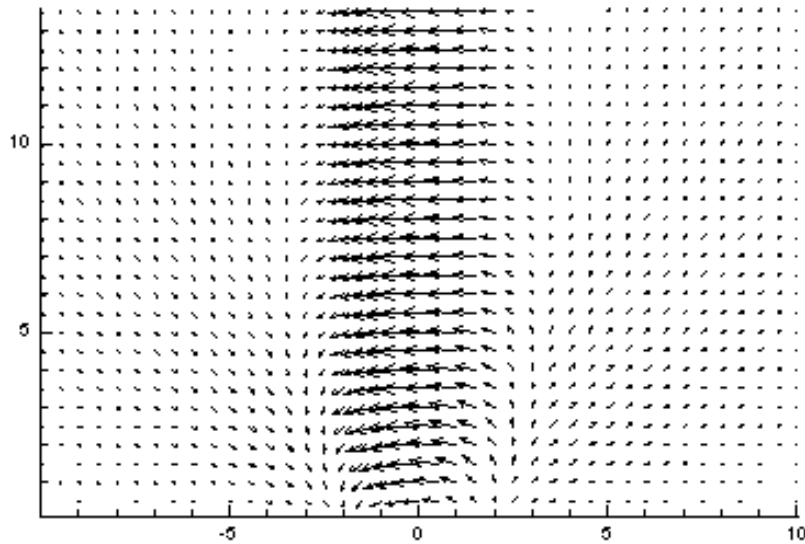
Figure 3. The perturbation velocity \hat{\mathbf{u}}_1 where \xi \in [-10, 10] \eta \in [0, 14]
