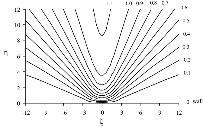
Figure 2. Dimensionless Streamline for \mathbf{w}_1 obtained from the stream function (56) with (60).
