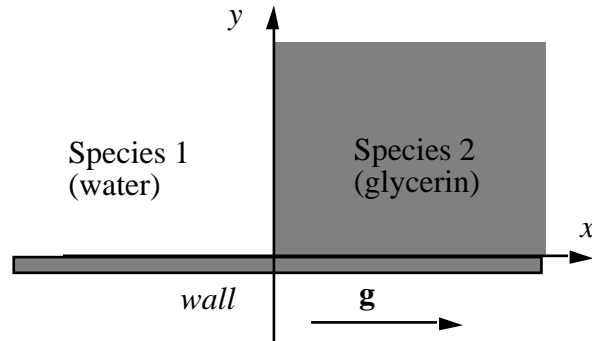
Figure 1. Two miscible liquids occupy the upper half plane. Initially, heavy fluid is on the right and light fluid is on the left with gravity \mathbf{g} = g\mathbf{e}_x in the direction of increasing x .
