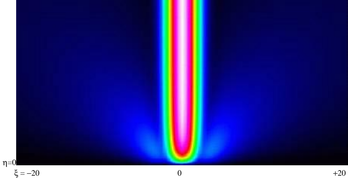
Figure 4. Contour plot of the velocity magnitude of the perturbation velocity \hat{\mathbf{u}}_1 within \xi \in [-20, 20] \eta \in [0, 20] . The black region has the magnitude 0; the blue region, about 0.1; the green region, about 0.5 and the white region has the maximal magnitude 1.0.
