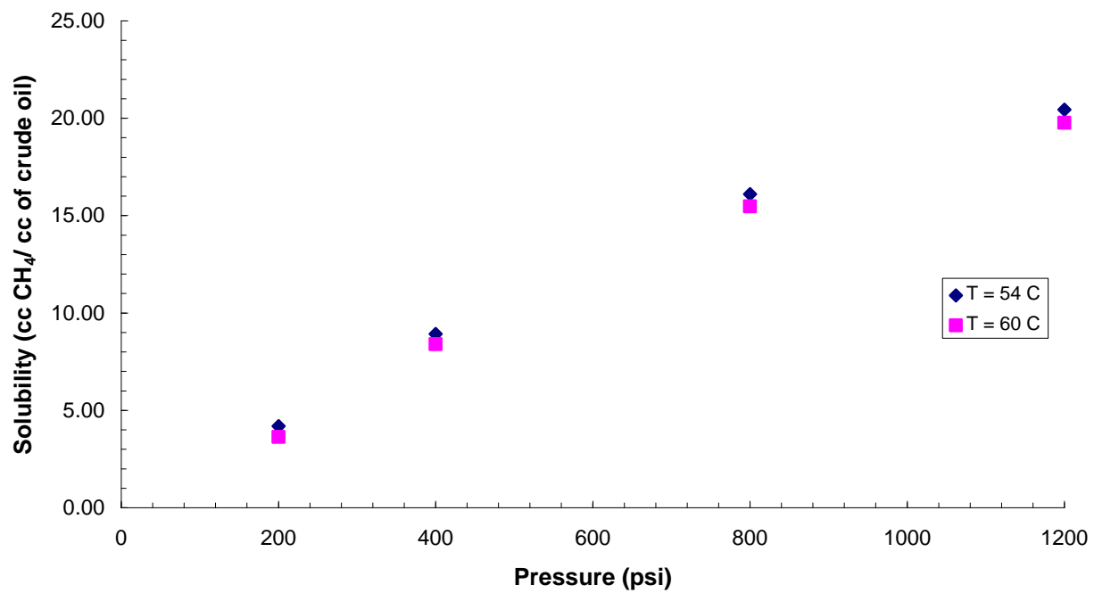
Methane solubility in Cerro Negro CrudeOil at 54 and 60 °C
