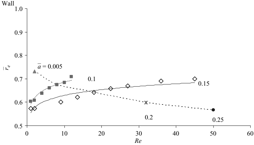
FIGURE 11. The stable equilibrium position \bar{r}_e of a neutrally buoyant sphere as a function of the Reynolds number. The two power law curves are for spheres with \bar{a} = 0.1 and \bar{a} = 0.15 , respectively. \diamond , \bar{r}_e = 0.555 Re^{0.0546} ; \blacksquare , \bar{r}_e = 0.591 Re^{0.0644} . All the points on the dotted line are for the same flow Reynolds number \bar{U}_m = 100 ; the dotted line shows that when \bar{U}_m is fixed, the equilibrium position becomes closer to the centreline as \bar{a} increases.
