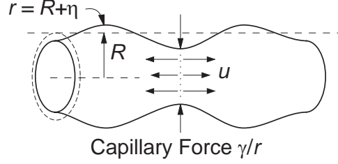
FIGURE 1. Capillary instability. The force \gamma/r drives fluid away from the neck, leading to collapse.
