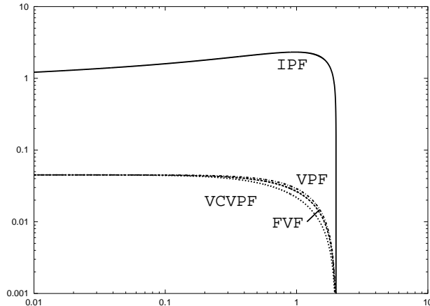
FIGURE 4. The growth rate \sigma vs. k for case 5 (inverse), air in SO10000. The growth rate by IPF is significantly larger than that by FVF; the results by VPF, VCVPF and FVF are almost the same (see table 2).
