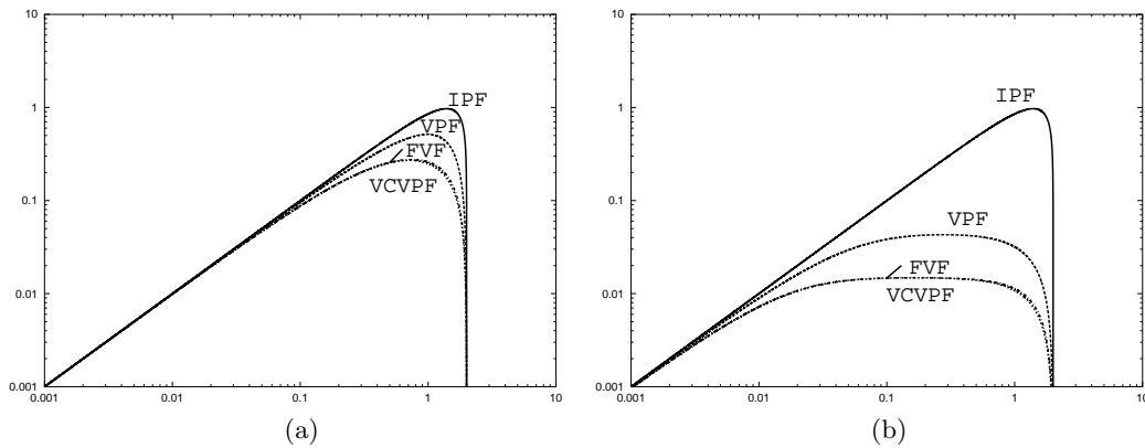
FIGURE 3. The growth rate \sigma vs. k for case 4, glycerine in air (a) and for case 5, SO10000 in air (b). The growth rates computed from IPF and VPF deviate considerably from the exact solution (FVF), but the growth rates from the corrected solution (VCVPF) are nearly the same as the exact solution (see table 2).
