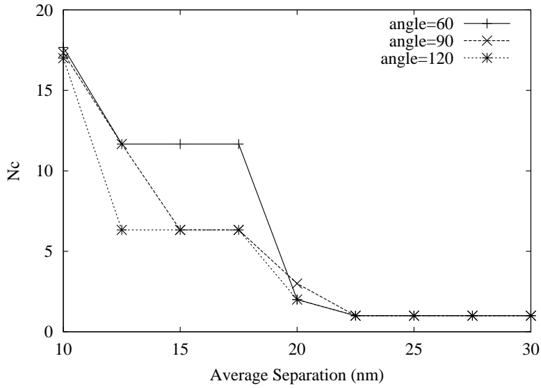
Figure 13: Effects of merging angle on N_c , the number of connected aircraft from the merge point, M_{hop} = 5 , \beta = 1 , and \sigma = 1 nm.
