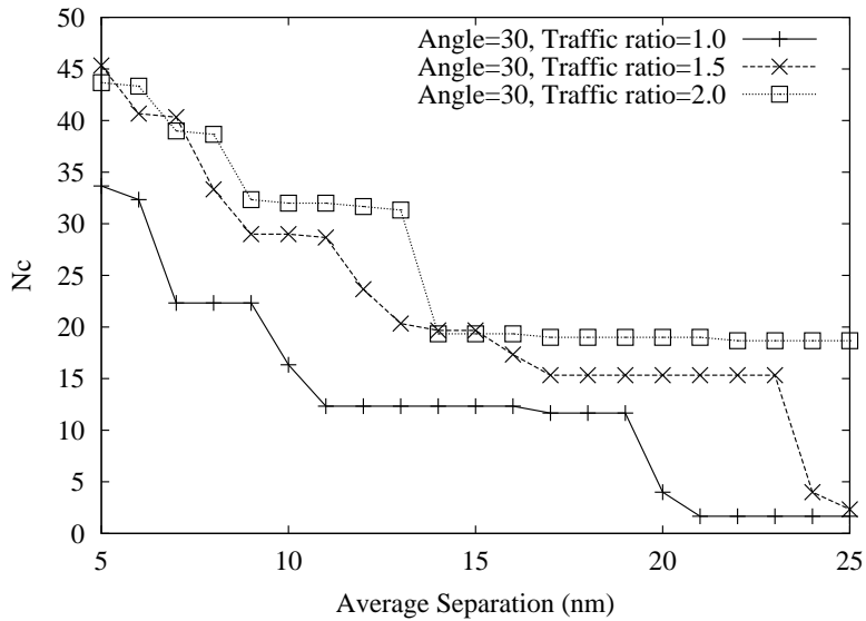
Figure 14: Effects of traffic ratio on N_c , the number of connected aircraft from the merge point, M_{hop} = 5 , \mu = 30 deg, and \sigma = 1 nm.
