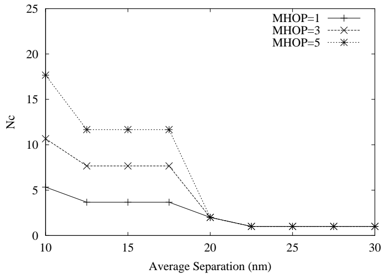
Figure 12: Effects of M_{hop} on N_c , the number of connected aircraft from the merge point, \mu = 60 deg, \beta = 1 , and \sigma = 1 nm.
