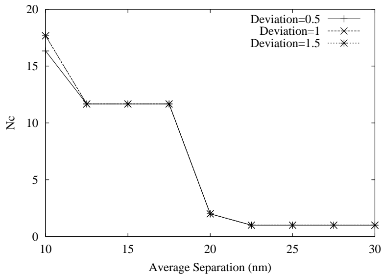
Figure 15: Effects of aircraft position uncertainty on N_c , the number of connected aircraft from the merge point, M_{hop} = 5 , \mu = 30 deg, and \beta = 1 .
